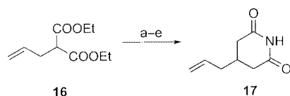
Scheme 4. Synthesis of allylglutarimide ( 17 ). Reagents and conditions: a) LiAlH 4 , Et 2 O, 0 °C to room temp. 12 h, 69%; b) p TsCl, KOH, THF, 0 °C, 2 h, then room temp., 4 h, 93%; c) NaCN, DMSO, 45 °C, 22 h; d) NaOH, MeOH, reflux, 4 h, 42% yield for the two steps; e) urea, 145 °C, 2 h, then 180 °C, 20 min; 73%. p TsCl = para -toluenesulfonyl chloride.
