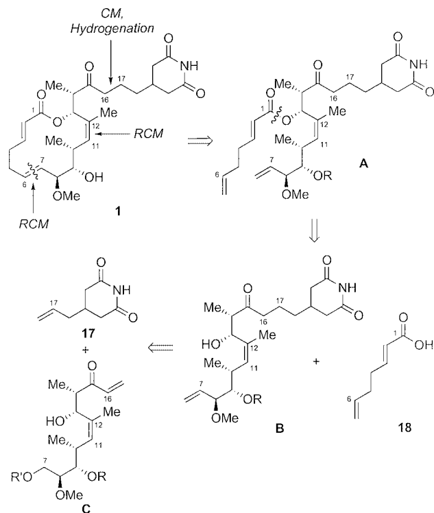
Scheme 1. Retrosynthetic plan for the synthesis of migrastatin ( 1 ). CM = Cross-Metathesis; RCM = Ring-Closing Metathesis.
