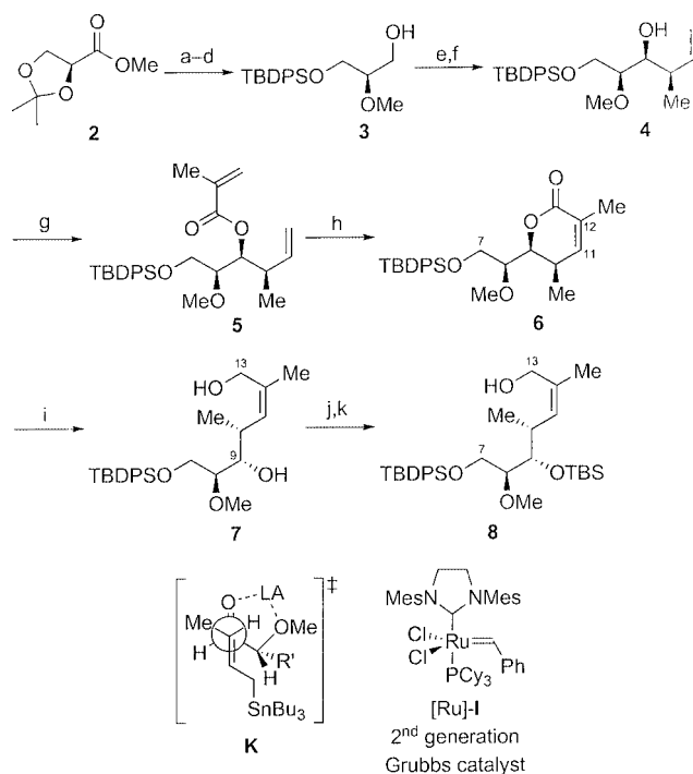
Scheme 3. Synthesis of alcohol 8 . Reagents and conditions: a) p TsOH, \text{MeOH}/\text{H}_2\text{O} (1:1), room temp., 83%; b) TBDPSCl, imidazole, \text{CH}_2\text{Cl}_2 , 0^\circ\text{C} to room temp. 81%; c) \text{Ag}_2\text{O} , MeI, MS 4 Å, \text{Et}_2\text{O} , 40^\circ\text{C} , 96%; d) DIBAL-H, \text{CH}_2\text{Cl}_2 , -78^\circ\text{C} to room temp. 90%; e) (\text{COCl})_2 , DMSO, \text{CH}_2\text{Cl}_2 , -78^\circ\text{C} , then \text{Et}_3\text{N} -78^\circ\text{C} to room temp.; f) \text{MgBr}_2\cdot\text{OEt}_2 , \text{CH}_2\text{Cl}_2 , -20^\circ\text{C} , then but-2-enyl-[(tri( n -butyl)]stannane, -60^\circ\text{C} , 87% (over two steps); g) methacryloyl chloride, \text{Et}_3\text{N} , DMAP, \text{CH}_2\text{Cl}_2 , 0^\circ\text{C} to room temp. 80%; h) [Ru]-I (16.5 mol-%), \text{CH}_2\text{Cl}_2 ( c = 10^{-2}\text{ M} ), 40^\circ\text{C} , 144 h, 65%; i) \text{LiBH}_4 (7 equiv.), \text{CeCl}_3\cdot 7\text{H}_2\text{O} (1 equiv.), \text{THF}/\text{H}_2\text{O} (4:1), room temp., 74%; j) TBSOTf, 2,6-lutidine, \text{CH}_2\text{Cl}_2 , 0^\circ\text{C} to room temp. 75%; k) \text{THF}/\text{H}_2\text{O}/\text{AcOH} (1:1:3), 36 h, room temp., 75%. p TsOH = para -toluenesulfonic acid; TBDPSCl = tert -butyldiphenylsilyl chloride; MS = molecular sieves; DIBAL-H = di-isobutylaluminum hydride; DMAP = 4-dimethylaminopyridine; TBSOTf = tert -butyldimethylsilyl trifluoromethanesulfonate.
