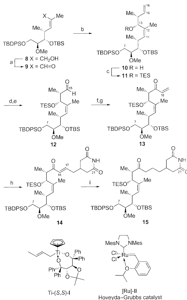
Scheme 5. Synthesis of fragment C7–C21 ( 15 ). Reagents and conditions: a) MnO 2 , CH 2 Cl 2 , room temp., 16 h; b) Ti-( S,S )- I , (1.4 equiv.), Et 2 O, –78 °C, 24 h, 80% over two steps; c) TESCl, CH 2 Cl 2 , room temp., 16 h, 90%; d) OsO 4 (4 mol-%), NMO (1 equiv.), t BuOH/H 2 O (1:1), room temp., 24 h; e) NaIO 4 (4.5 equiv.), THF/H 2 O (1:1), room temp., 10 h, 80% over two steps; f) vinylmagnesium chloride (3 equiv.), –78 °C, THF, 0.5 h; g) Dess–Martin periodinane (2 equiv.), CH 2 Cl 2 , 0 °C to room temp. 1 h, 73% over two steps; h) [Ru]- II (30 mol-%), 17 (3 equiv.), CH 2 Cl 2 , room temp., 10 h, 32%; i) Pd/C 5% (5 mol-% Pd), EtOAc, room temp., 10 h, 96%. TESCl = triethylsilyl chloride, NMO = N -methyl-morpholine N -oxide.
