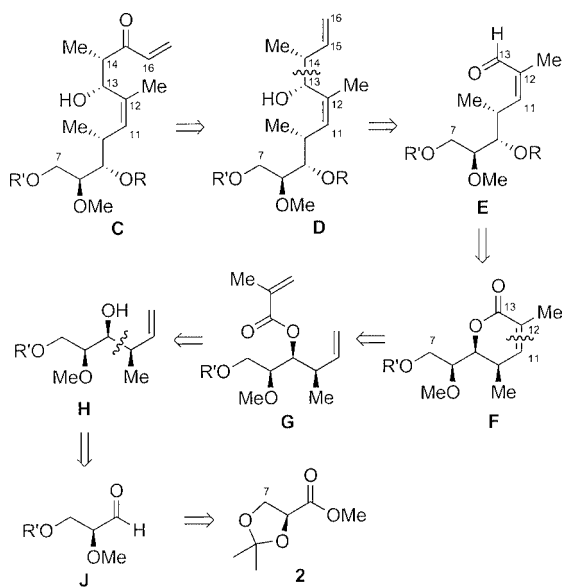
Scheme 2. Retrosynthetic analysis of fragment C (C7–C16).
