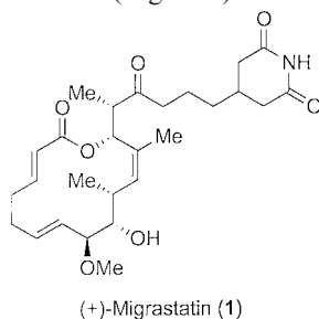
Figure 1. Structure of migrastatin (1).
